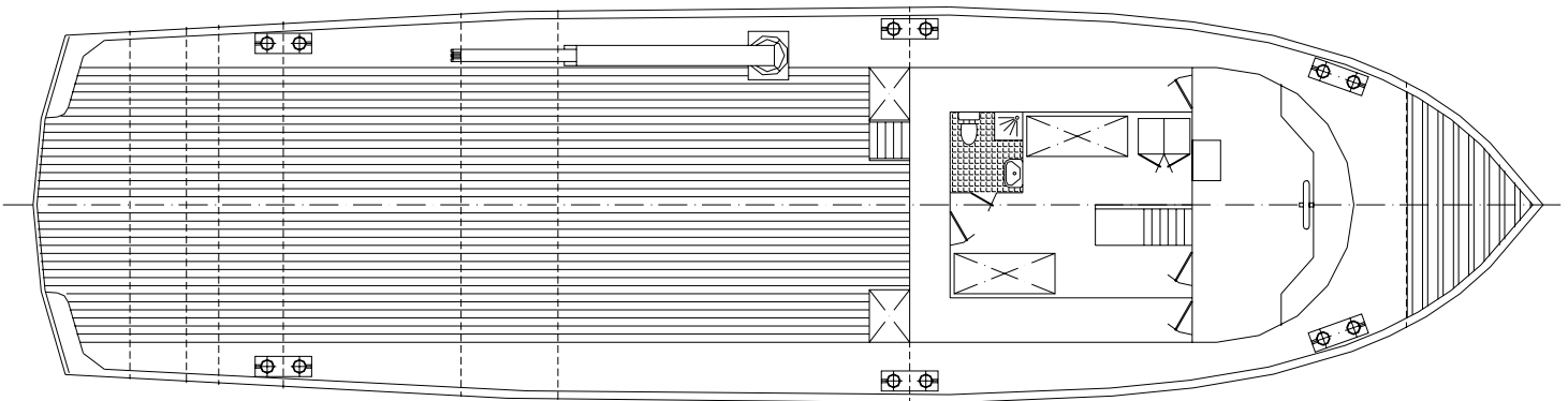
MAIN DECK
