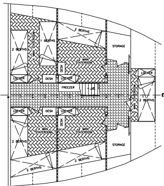
ACCOMMODATION BELOW DECK
