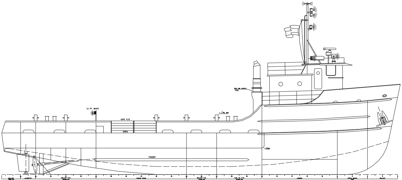
OUT BOARD PROFILE
